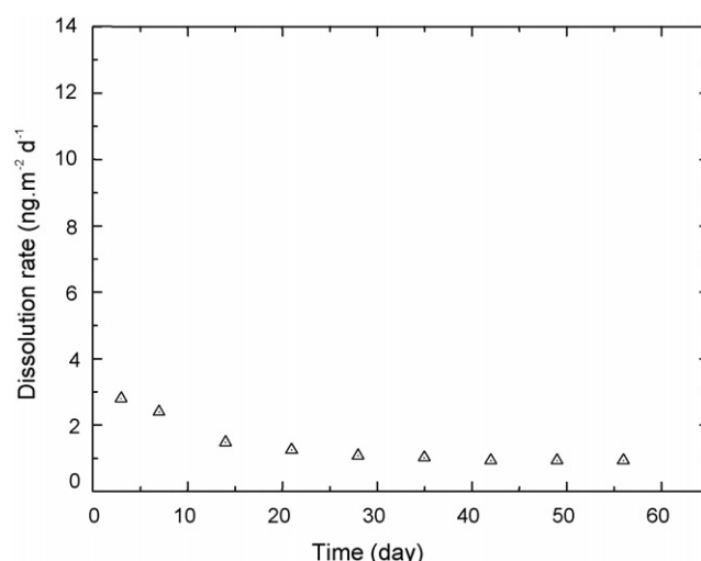
Fig. 3. Powder leaching results on perlite charged by 10 wt.% in \text{Cs}_2\text{O} .
