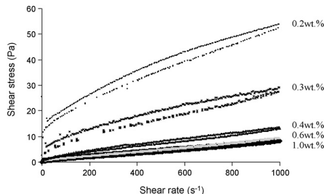
Fig. 2. Flow curves of 30 vol.% slips prepared in EtOH with EPH as deflocculant.
