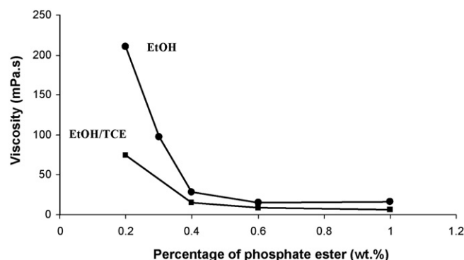
Fig. 3. Variation of viscosity of 30 vol.% slips prepared in EtOH and TCE/EtOH with EPH content.
