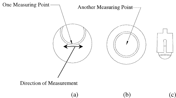
Fig. 1. Residual stress measuring points.
