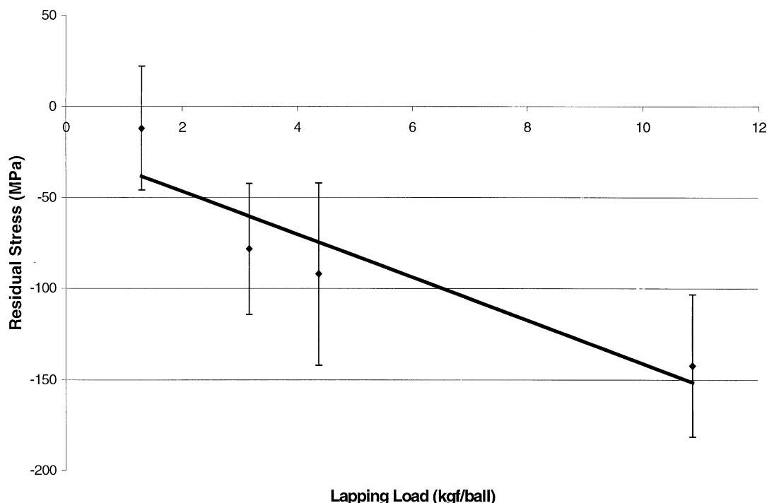
Fig. 2. Residual stress versus lapping load.
