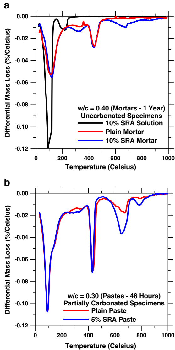
Fig. 11. Thermogravimetric analysis of: (a) uncarbonated cement mortars with and without SRA, along with that of a bulk SRA solution. The mass values for the solution have been divided by a factor of 10 to appear on the same scale as the mortar datasets and (b) partially carbonated cement pastes with and without SRA [33,61].
