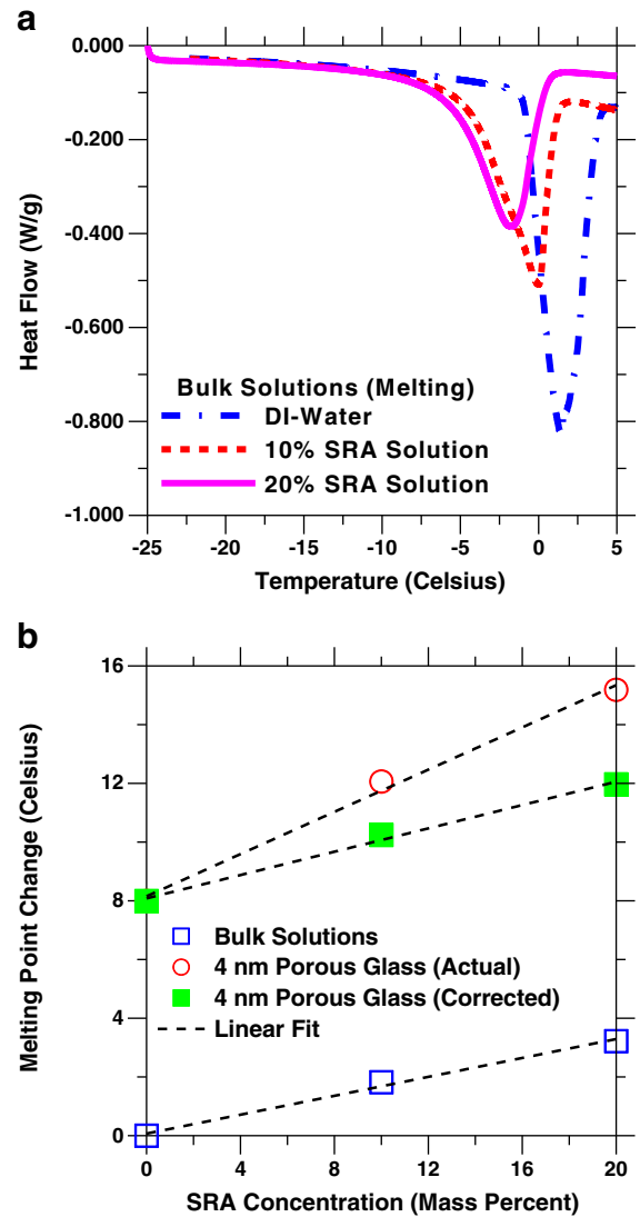
Fig. 7. (a) Melting curves for solutions of de-ionized water and a solution containing SRA and (b) the influence of the SRA on the melting point change of bulk water and SRA solutions and solutions contained in the 4 nm porous glass.
