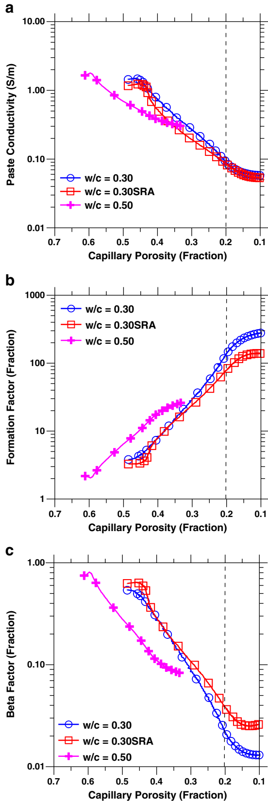
Fig. 9. (a) The electrical conductivity as a function of the capillary porosity, (b) The formation factor as a function of the capillary porosity and (c) The Beta factor (moisture connectivity) as a function of the capillary porosity. The dashed line on the graphs indicates the capillary porosity-based depercolation threshold proposed by Powers and co-workers [15,16].
