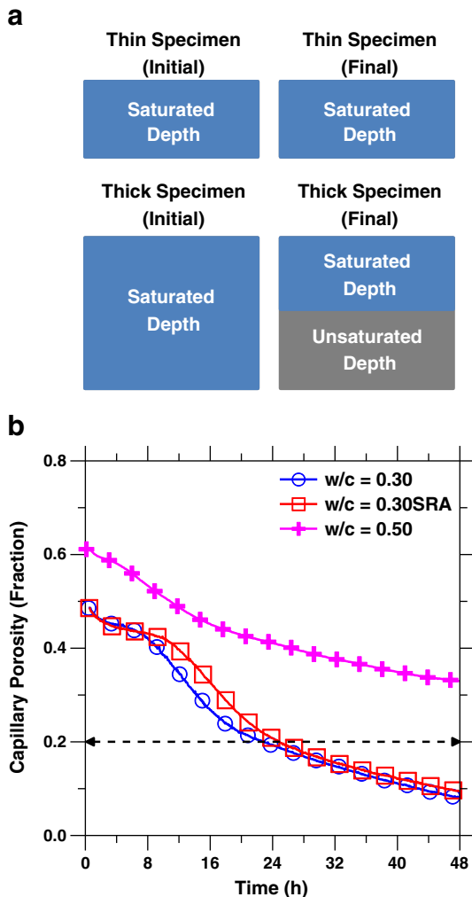
Fig. 8. (a) An illustration of the change in the degree of fluid saturation as a function of depth and hydration in thin and thick specimens and (b) The capillary porosity as a function of time. The dashed line indicates the depercolation threshold proposed by Powers and co-workers [15,16].
