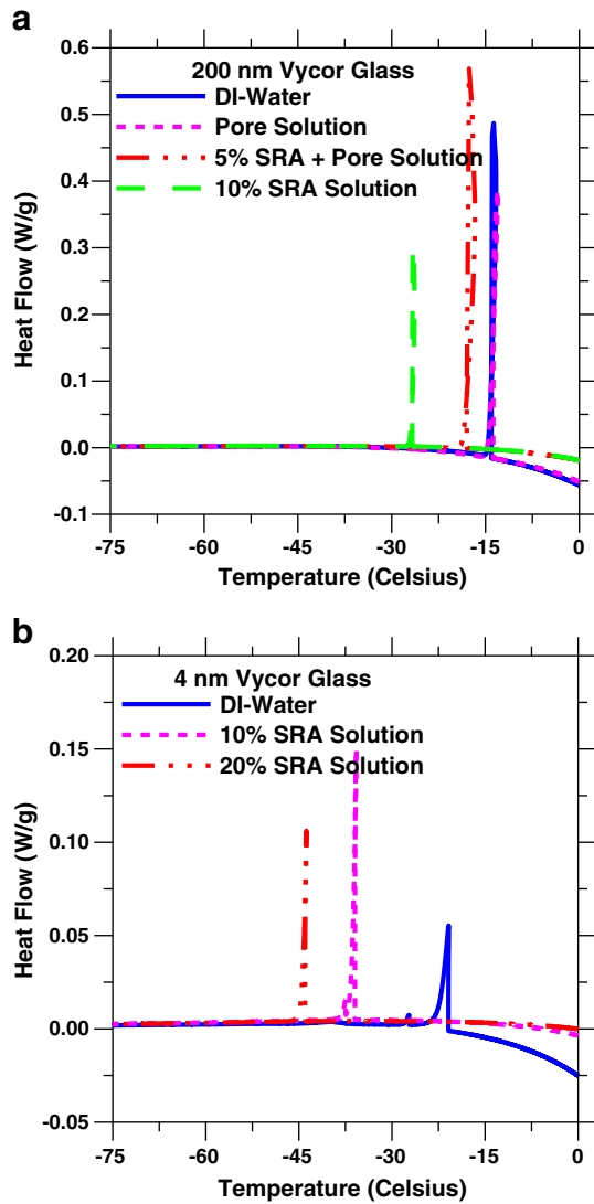
Fig. 6. LTC scans for porous glasses saturated with solutions with and without a SRA for: (a) 200 nm porous glass and (b) 4 nm porous glass.
