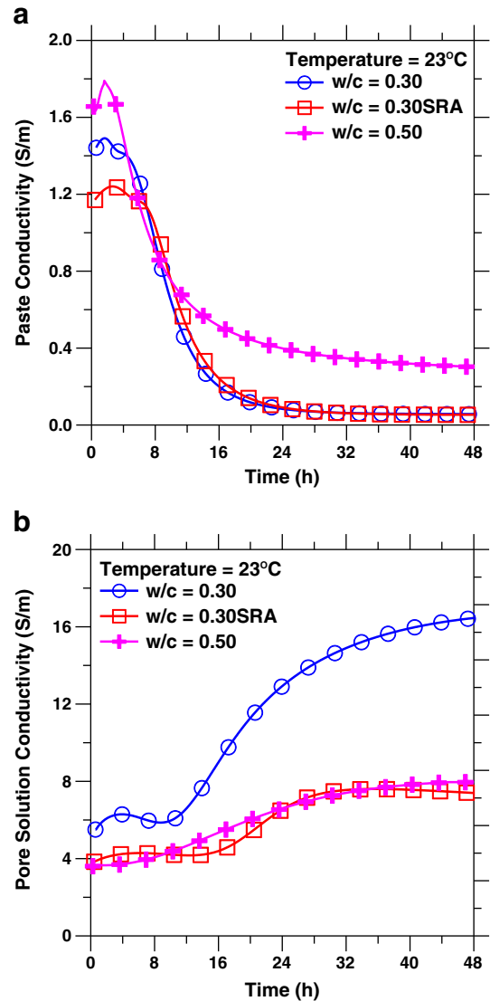
Fig. 3. The measured electrical conductivity measured as a function of specimen age for: (a) cement pastes and (b) extracted pore solutions.
