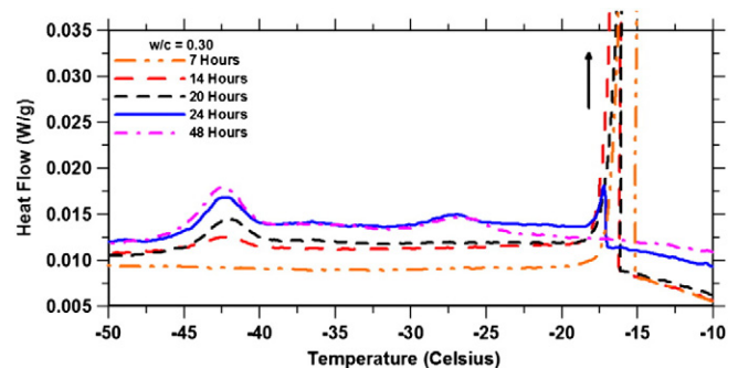
Fig. 4. Representative LTC Scans for a plain cement paste ( w/c = 0.30 ) at several ages.
