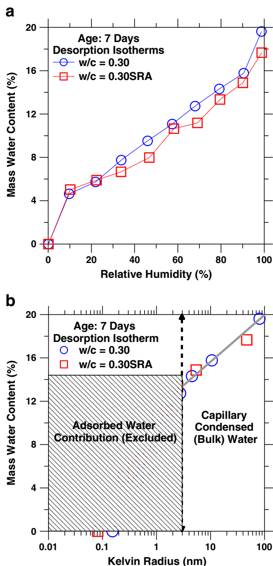
Fig. 10. (a) The first desorption isotherm for plain and 5% SRA containing cement pastes and (b) The governing Kelvin radius as a function of the desorbed water content, wherein, the Kelvin radius is determined after considering the influence (reduction) of the SRA on the surface tension at the liquid–vapor interface. 6 The dashed line shows the dimensional thermodynamic stability limit of the interfacial liquid–vapor meniscus at a Kelvin Radius of around 3 nm [8,62–64].
