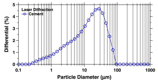
Fig. 1. The particle size distribution of the cement used in this investigation as measured using laser diffraction. The results shown are the average of six individual measurements and the error bars (one standard deviation) would fall well within the size of the shown symbols.
