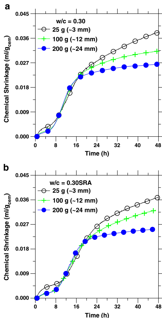
Fig. 2. Chemical shrinkage as a function of specimen age for cement paste mixtures for specimens of varying thicknesses: (a) w/c = 0.30 and (b) w/c = 0.30\text{SRA} .
