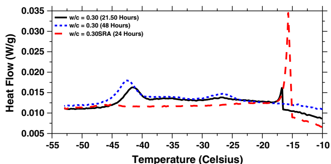
Fig. 5. Representative LTC scans for cement pastes illustrating the persistence of the -15^{\circ}\text{C} freezing peak in SRA containing pastes.
